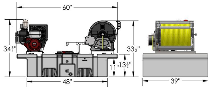
Above picture shows 21-87UVXX-P530 with 53-HAE1526-1 and 23-850000 Boom
