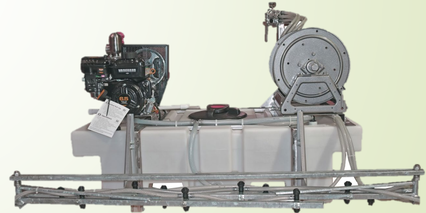
16FT BREAK AWAY BOOM MANUAL CONTROLS
